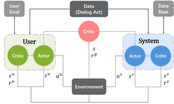
Figure 2: Architecture of MADPL. HVN consists of three critics. Each critic estimates its return based on role-aware reward decomposition, and each actor uses the estimated value to optimize itself.
