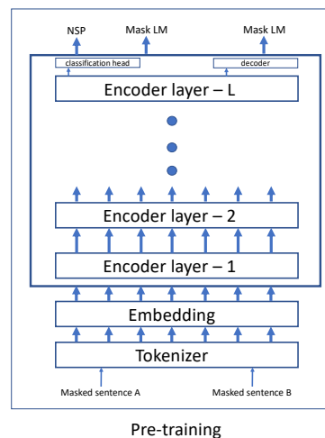
Figure 1: BERT pre-training
