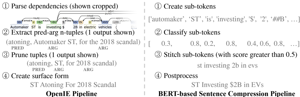
Figure 3: Illustrations of the symbolic OpenIE (left) and neural sentence compression (right) candidate extraction pipelines. We apply both, to render a diverse pool of candidate summaries, and use a ranker to select the best.
