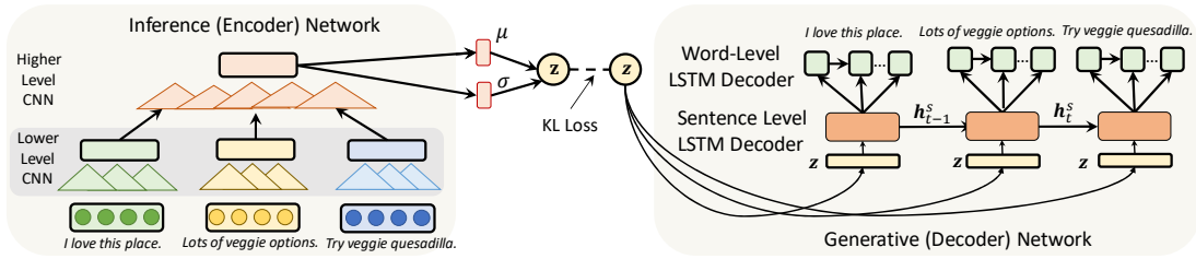
Figure 3: Schematic diagram of the proposed multi-level VAE with single latent variable.
