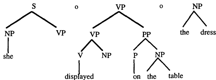
Figure 4. Another derivation generating the same tree for "She displayed the dress on the table"
