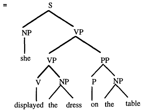
Figure 2. Derivation and parse tree for "She displayed the dress on the table"
