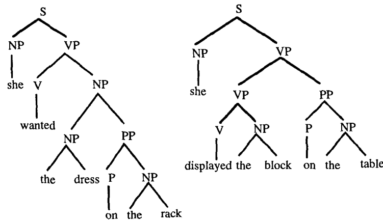
Figure 1. Example corpus of two trees.
