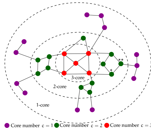
Figure 2: k -core decomposition of a graph and illustration of the value added by CoreRank. While nodes * and ** have the same core number ( =2 ), node * has a greater CoreRank score ( 3+2+2=7 vs 2+2+1=5 ), which better reflects its more central position in the graph.
