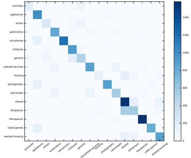
Figure 1: Confusion Matrix
