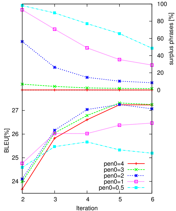
Figure 2: BLEU scores and percentage of surplus phrases on dev over the first 6 training iterations with different backoff phrase penalties pen_0 .
