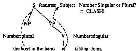
Figure 2. Co-occurrence Restrictions are Enforced by Feature Checking in an LFG.
