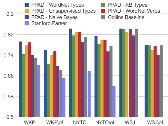
Figure 4: PPAD variations vs. baselines.
