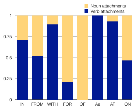
Figure 3: Noun vs. verb attachment proportions for frequent prepositions in the labeled NYTC dataset.
