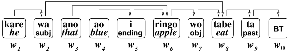
Figure 1: Dependency structure of a sentence.
