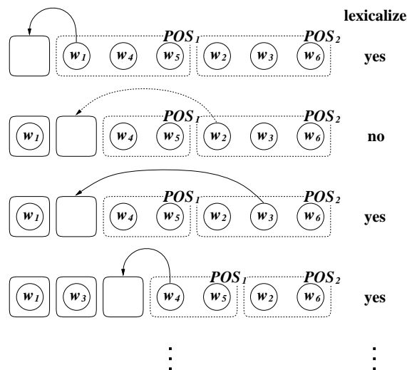
Figure 3: A conceptual figure of the lexicalization algorithm.
