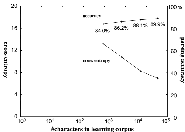
Figure 4: Relation between cross entropy and parsing accuracy.
