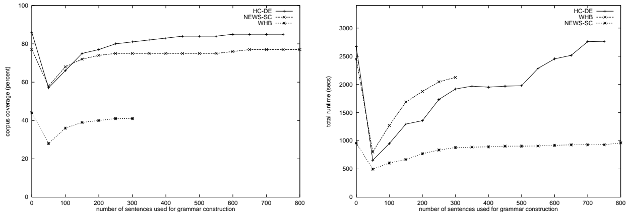
Figure 8: Performance of fragment grammars
