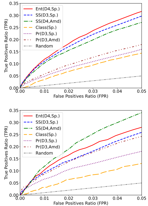
Figure 2: ROC curves ( FPR \leq 0.05 region) for the Retweet dataset (Top) and Meetings dataset (Bottom)
