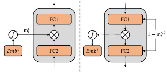
Figure 3: Illustration of new domain learning: forward (the left) and backward (the right) propagation. Here, we show the inner structure of the feed-forward layer.
