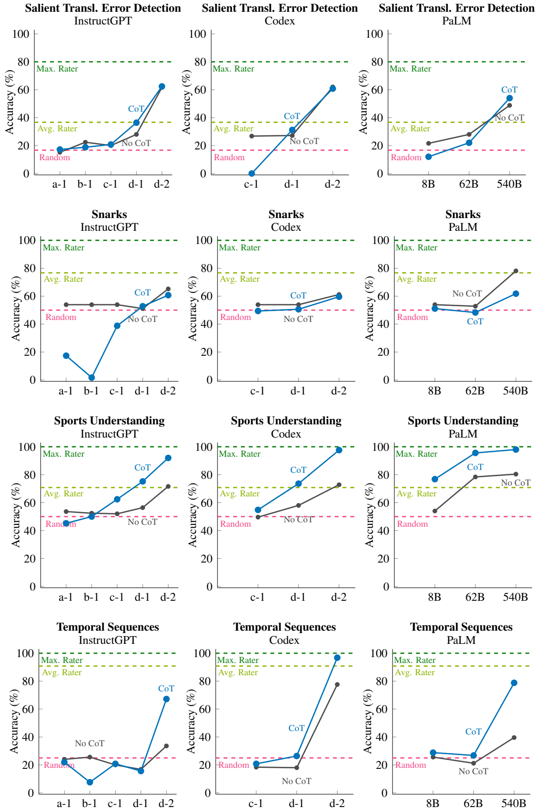
Figure 12: Salient Translation Error Detection, Snarks, Sports Understanding, and Temporal Sequences.
