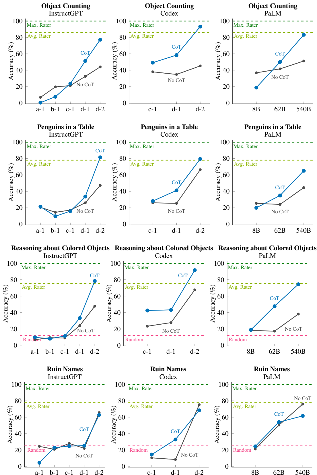
Figure 11: Object Counting, Penguins in a Table, Reasoning about Colored Objects, and Ruin Names.
