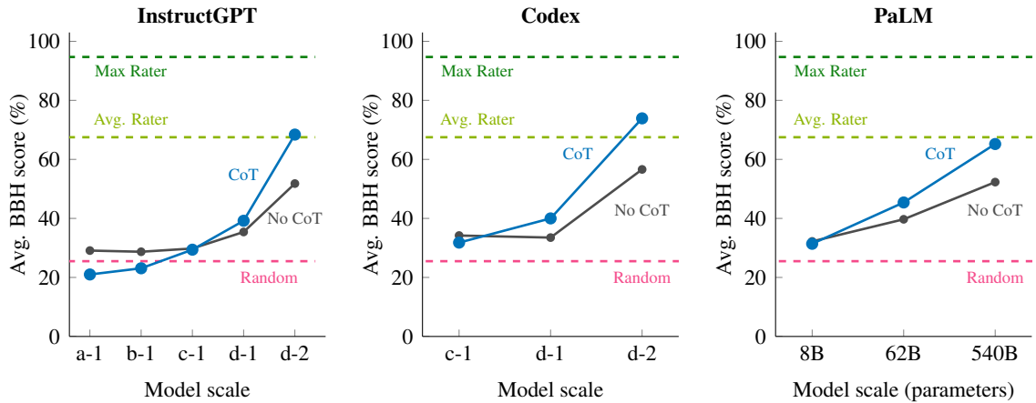
Figure 4: Scaling behavior of CoT prompting on BIG-Bench Hard (BBH; 23 task unweighted average). InstructGPT models are the following: a-1 (text-ada-001), b-1 (text-babbage-001), c-1 (text-curie-001), d-1 (text-davinci-001), and d-2 (text-davinci-002). Codex models are the following: c-1 (code-cushman-001), d-1 (code-davinci-002), and d-2 (code-davinci-002).
