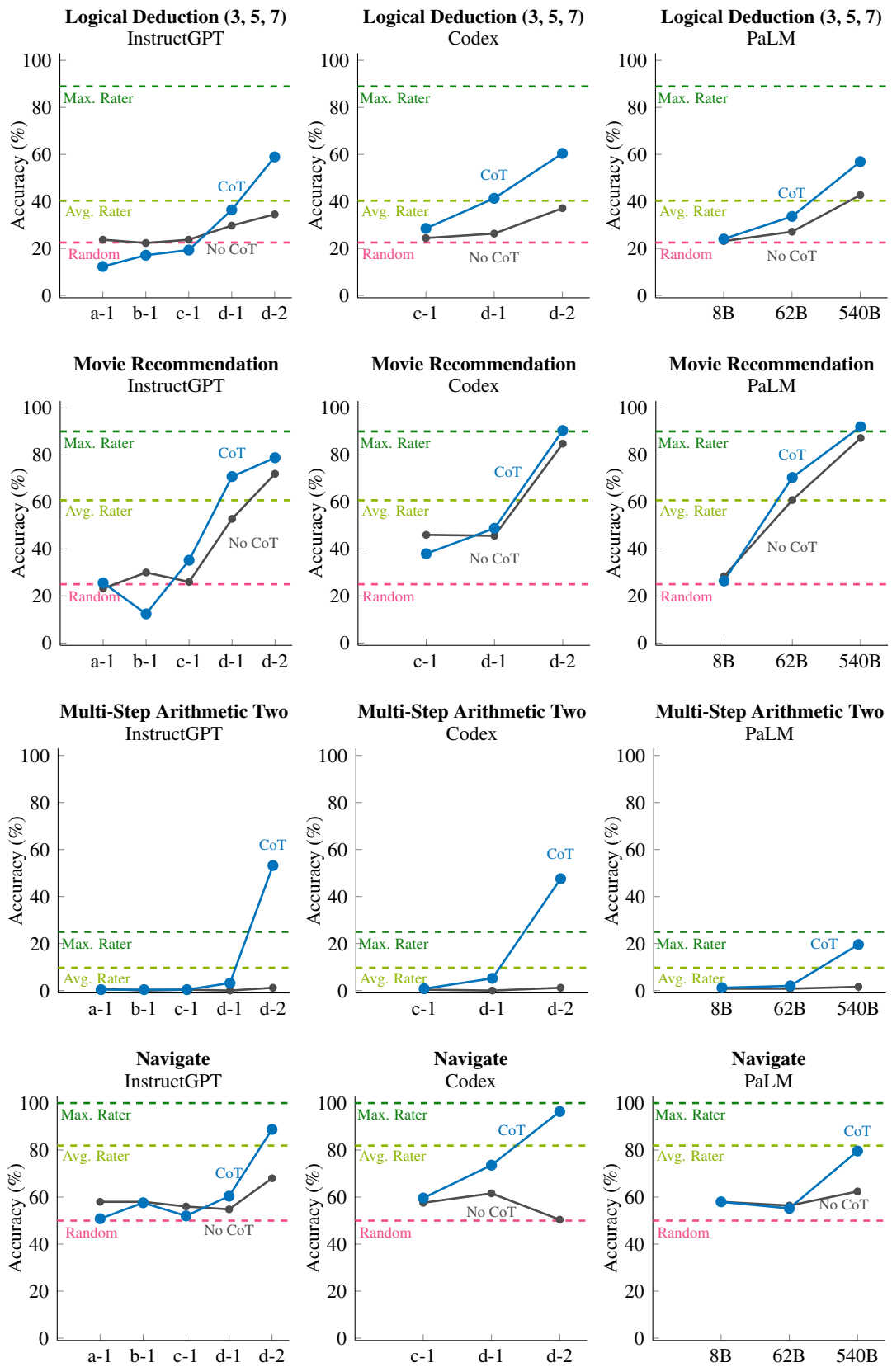
Figure 10: Logical Deduction, Movie Recommendation, Multi-Step Arithmetic (Two), and Navigate.
