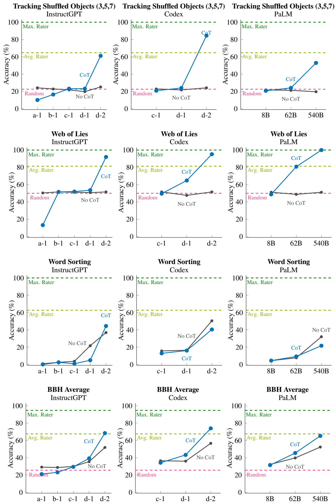
Figure 13: Tracking Shuffled Objects, Web of Lies, Word Sorting, and BBH All Average.
