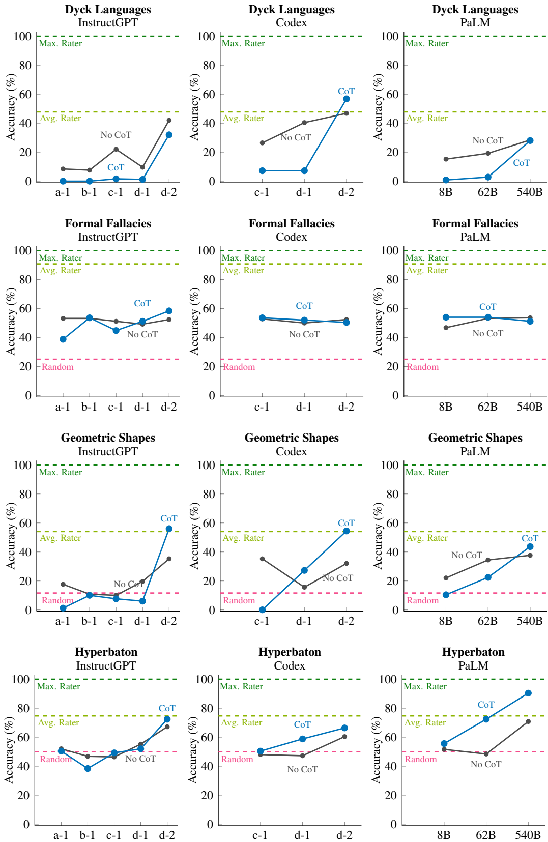
Figure 9: Dyck Languages, Formal Fallacies, Geometric Shapes, and Hyperbaton.
