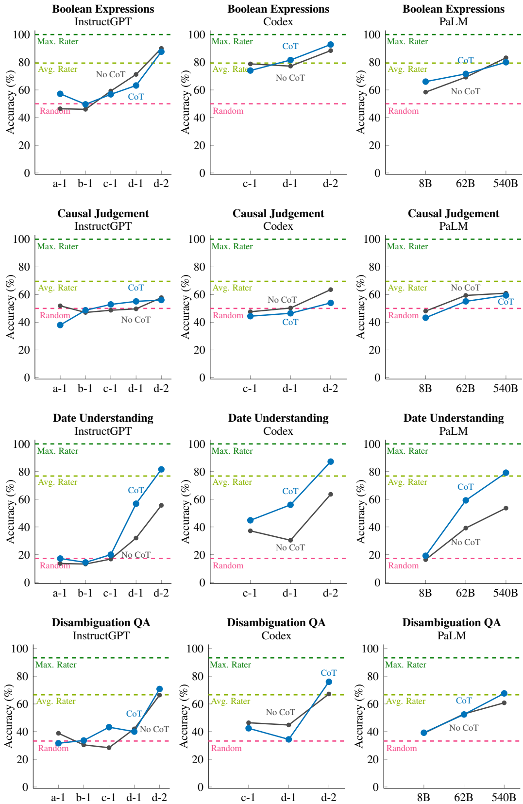
Figure 8: Boolean Expressions, Causal Judgement, Date Understanding, and Disambiguation QA.
