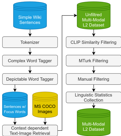
Figure 2: Schematic overview of the dataset collection pipeline.
