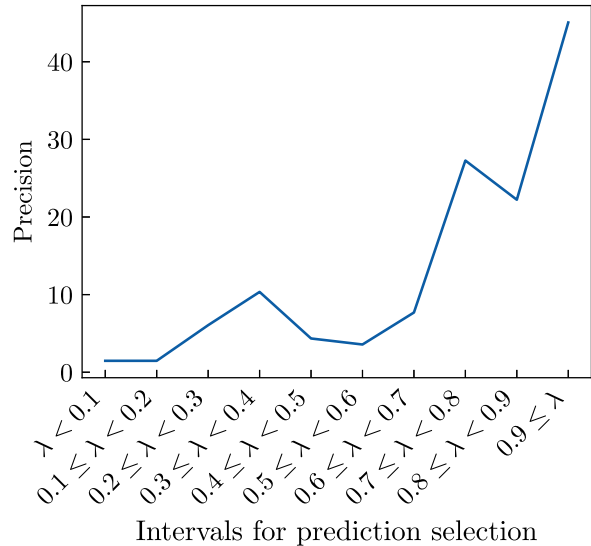
Figure 3: Precision differences in varying threshold ranges.
