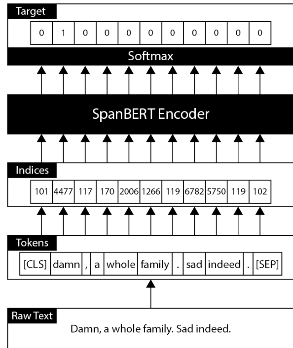
Figure 2: The flowchart of SpanBERT-based model
