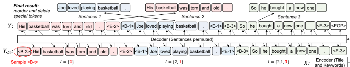
Figure 3: The decoding process during inference as described in Section 4.3. Note that the first special token (e.g., <B-2>) is sampled from \{\langle B-t \rangle\}_{t=1}^T . For simplicity, positional embedding is omitted in the figure.
