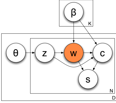
Figure 2: Our generative model assumes that documents are divided into topics and that these topics generate both the observed word and a “corroborator,” a term similar in usage to the word. Next, a sense that minimizes the semantic distance between the corroborator and the word is generated.
