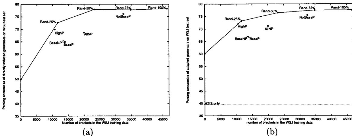
Figure 2: Parsing accuracies of (a) directly induced grammars and (b) adapted grammars as a function of the number of brackets present in the training corpus. There is a total of 46463 brackets in the training corpus.
