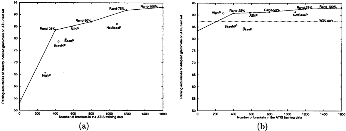
Figure 1: Parsing accuracies of (a) directly induced grammars and (b) adapted grammars as a function of the number of brackets present in the training corpus. There are 1595 brackets in the training corpus all together.
