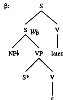
Figure 5: Verb-raising tree in Dutch.
