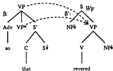
Figure 3: Wrapping athematic tree.
