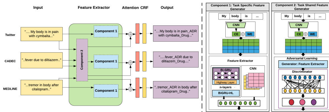
Figure 2: Proposed model architecture for pharmacovigilance mining. (all the neurons representation are hypothetical). The right part of the image describes the Component 1 and Component 2 .
