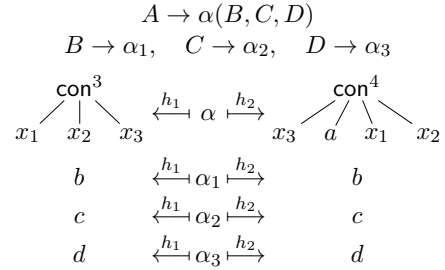
Figure 2: An IRTG encoding an SCFG.
