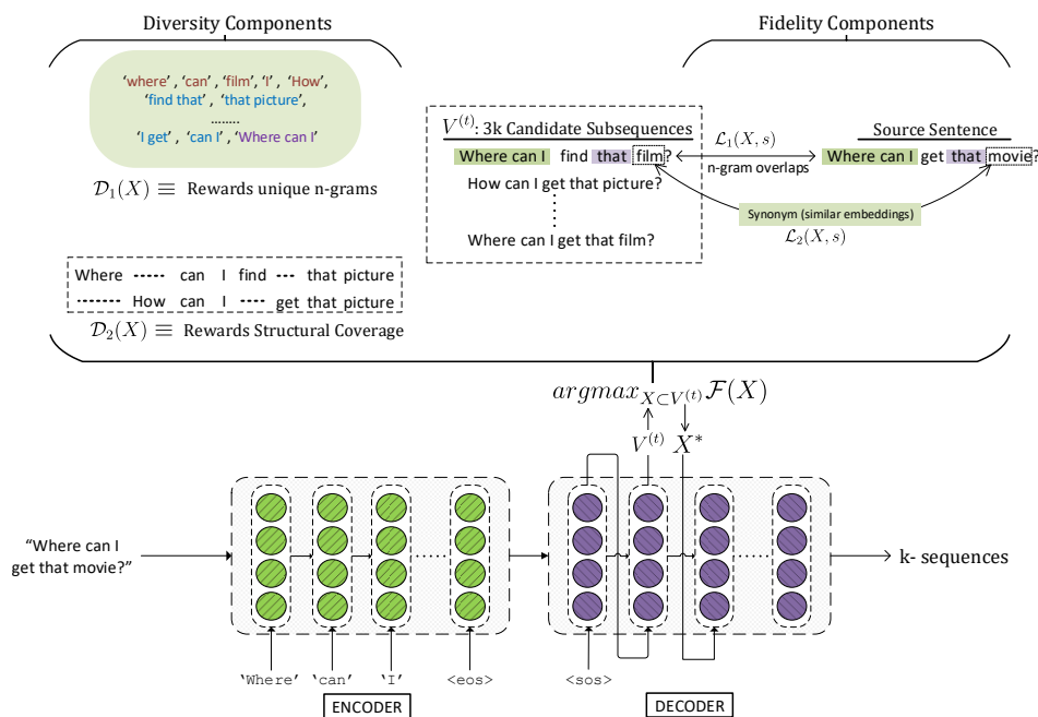
Figure 1: Overview of DiPS during decoding to generate k paraphrases. At each time step, a set of N sequences ( V^{(t)} ) is used to determine k < N sequences ( X^* ) via submodular maximization. The above figure illustrates the motivation behind each submodular component. Please see Section 4 for details.
