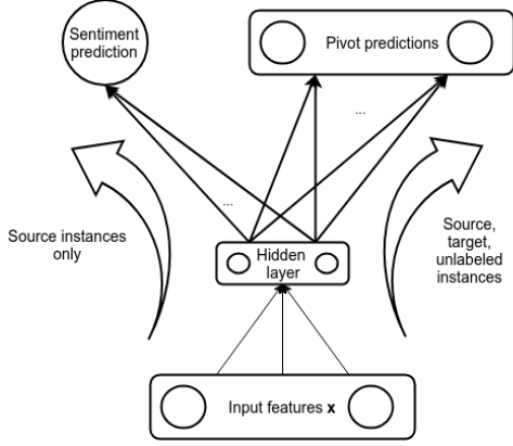
Figure 1: Network architecture for unsupervised domain adaptation.
