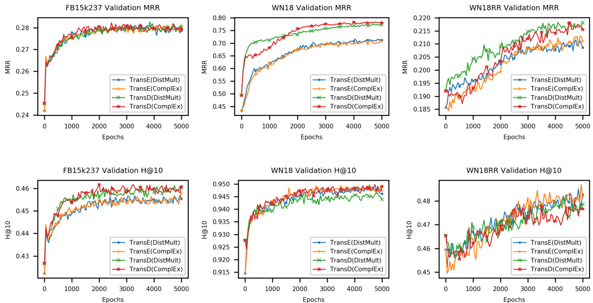
Figure 2: Learning curves of KBGAN. All metrics improve steadily as training proceeds.
