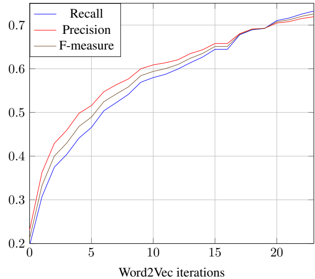
Figure 2: Evolution of the Recall, Precision and F-measure for each Word2Vec iterations
