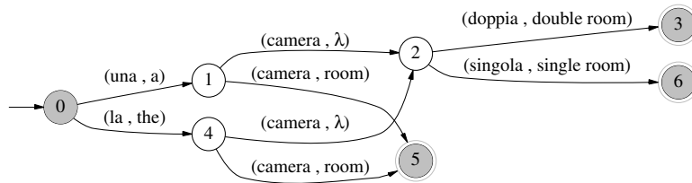
Figure 4 Bigram model inferred from strings obtained by the transformation \mathcal{L}_1 in example 2.
