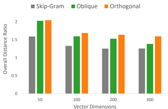
Figure 3: Overall distance ratio ( DR_{overall} ) over word vector dimensions. The rotated vectors (parsimax-obtogonal and varimax-oblique) show higher DR_{overall} score than the original skip-gram vectors.
