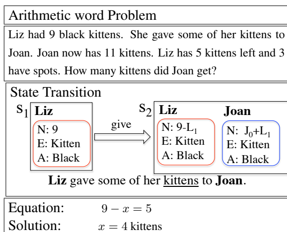
Figure 1: Example problem and solution.
