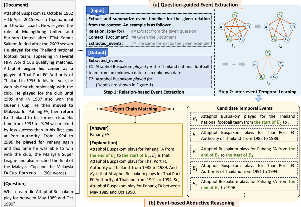
Figure 2: The overall framework of Event-AL. It consists of a question-guided event extraction module for capturing and completing candidate temporal events related to the question, and an event-based abductive reasoning module for obtaining and checking answers.
