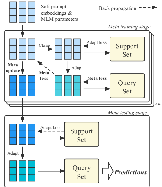
Figure 3: Meta training and testing procedures of MetaPrompting.
