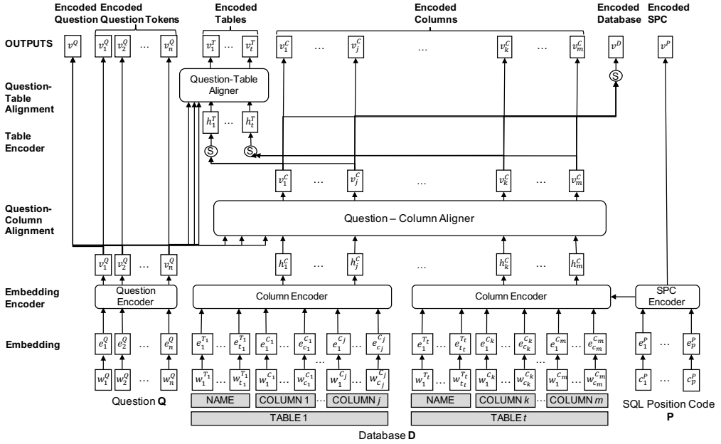
Figure 2 Network architecture of the proposed input encoder. Ⓢ represents self-attention.
