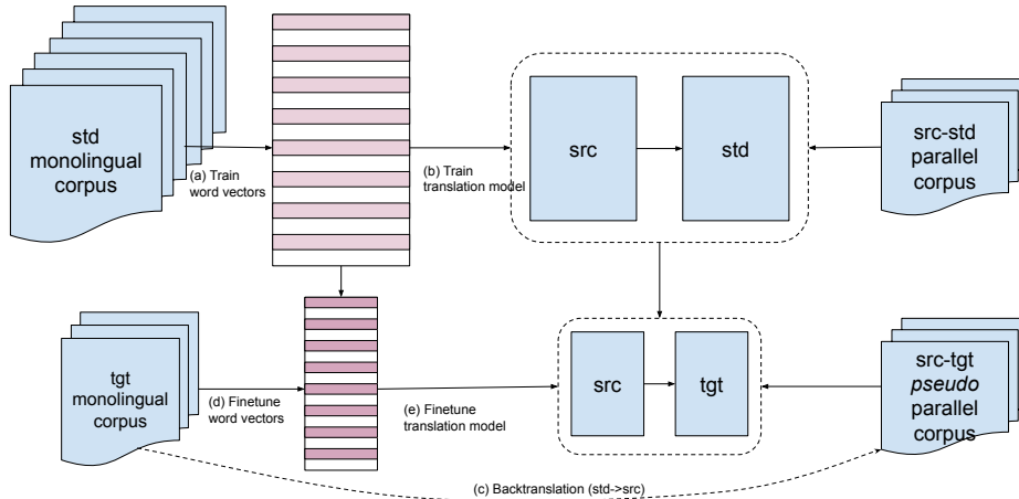
Figure 1: An overview of our approach. (a) Using the available STD monolingual corpora, we first train word vectors using fasttext ; (b) we then train a SRC→STD translation model using the parallel corpora to predict the pretrained word vectors; (c) next, we train STD→SRC model and use it to translate TGT monolingual corpora to SRC; (d) now, we finetune STD subword embeddings to learn TGT word embeddings; and finally (e) we finetune a SRC→STD model to generate TGT pretrained embeddings using the back-translated SRC→TGT data.
