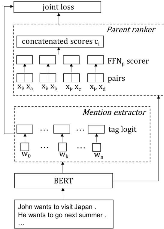
Figure 2: Model architecture for the joint model. The input is a document, which is a list of sentences. x_i is the child node. For simplicity, we consider x_a, x_b, x_c, x_d as the candidate parent nodes.
