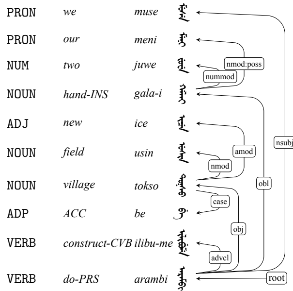
Figure 1: Dependency Tree for ‘We construct the new countryside with our two hands’.
