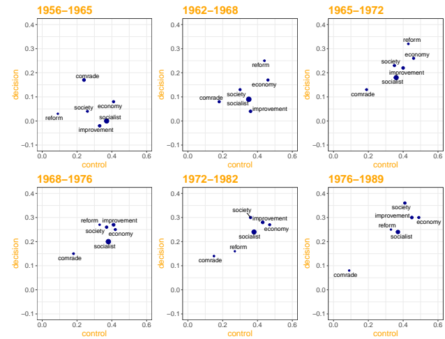
Figure 3: Changes in the cosine similarity of the concepts examined over time.
