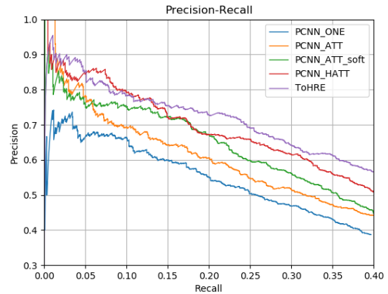
Figure 4: Precision-recall curves.
