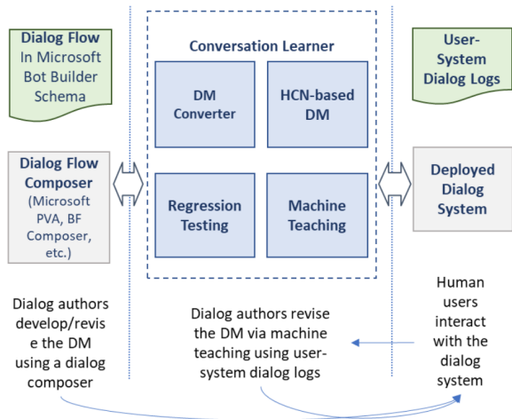
Figure 2: The architecture of Conversation Learner (Top) and the development of DMs using Conversation Learner (Bottom).
