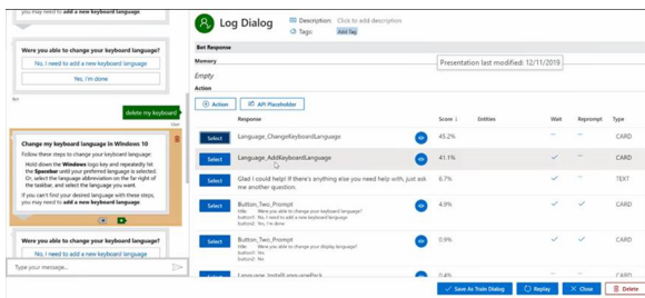
Figure 7: Machine Teaching UI for correcting dialogs to revise DM.
