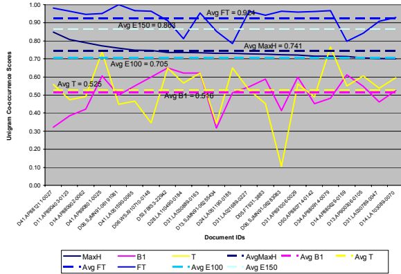
Figure 6. DUC 2001 single document inter-human, baseline, system, and full text unigram co-occurrence score distributions (Set A).
