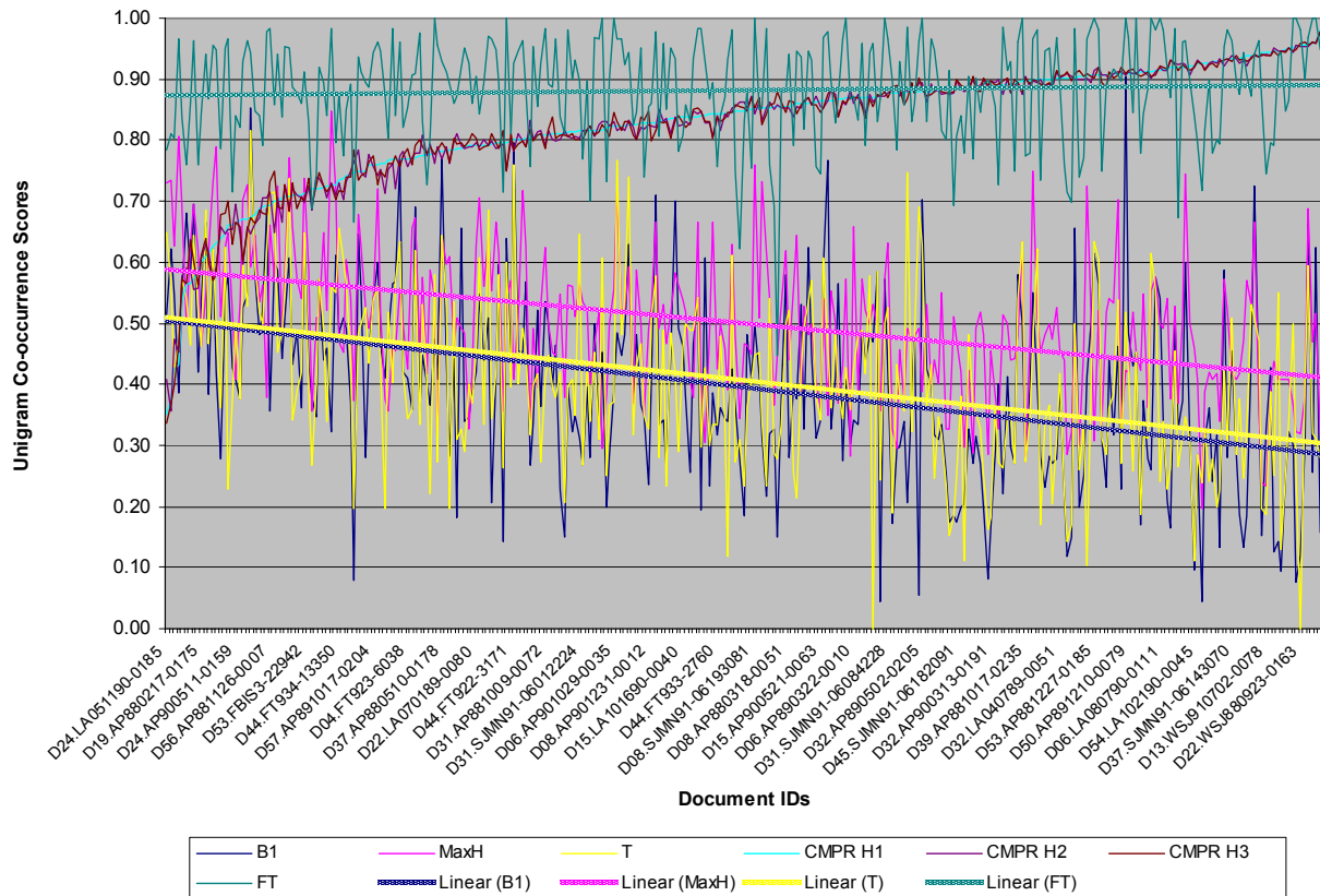
Figure 9. DUC 2001 single doc inter-human, baseline, and system unigram co-occurrence score versus compression ratio. Document IDs are sorted by increasing compression ratio CMPR H1.
