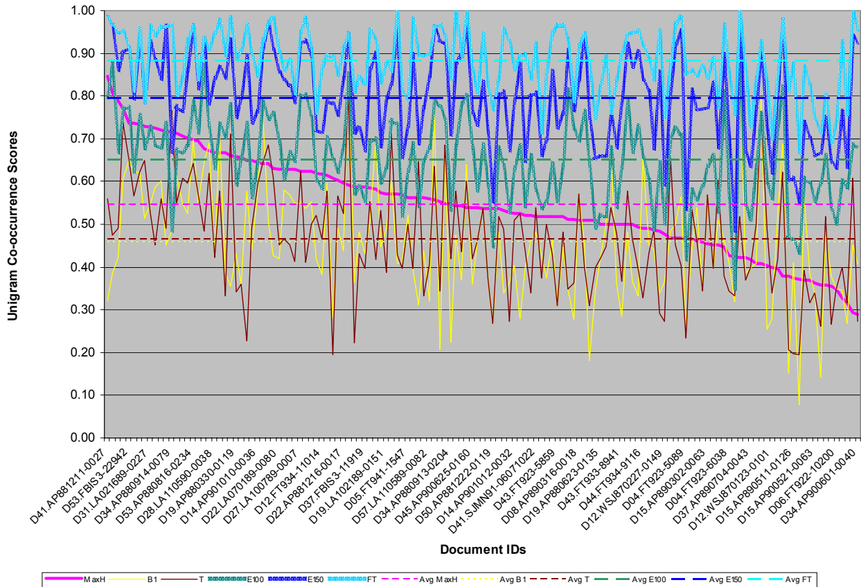
Figure 5. DUC 2001 single document inter-human, baseline, system, 100-word, 150-word, and full text oracle extracts unigram co-occurrence score distributions (# of sentences \leq 30 ). Document IDs are sorted by decreasing MaxH.
