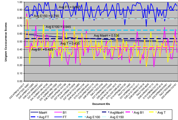
Figure 8. DUC 2001 single document inter-human, baseline, system, and full text unigram co-occurrence score distributions (Set C).
