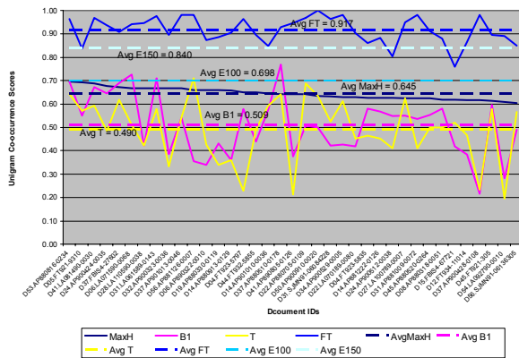
Figure 7. DUC 2001 single document inter-human, baseline, system, and full text unigram co-occurrence score distributions (Set B).
