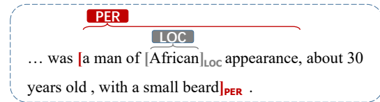
Figure 5: A representative error case of ARNs, where the right boundary of the PER mention is misclassified. Braces above the sentence indicate the output of ARNs, and brackets in the sentence represent the golden annotation. We find that the majority of errors occur because of the long-term dependencies stemming from postpositive attributive and attributive clauses.
