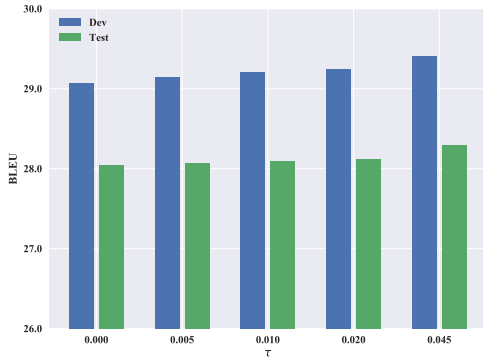
(a) Machine translation
