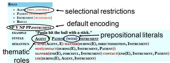
Figure 2: Information associated with a VerbNet frame entry.
