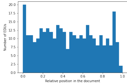
Figure 6: Distribution of relative positions of the most impactful EDUs for the left class ( Allsides ).
