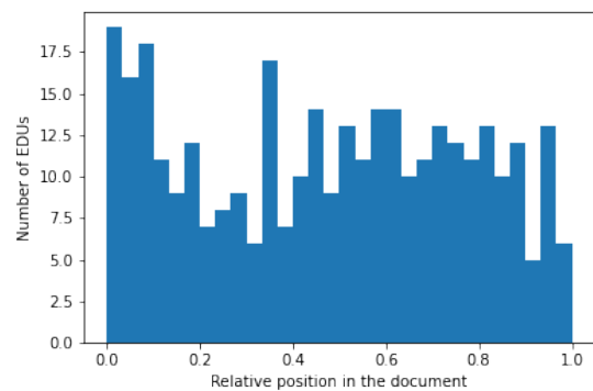
Figure 8: Distribution of relative positions of the most impactful EDUs for the right class ( Allsides ).
