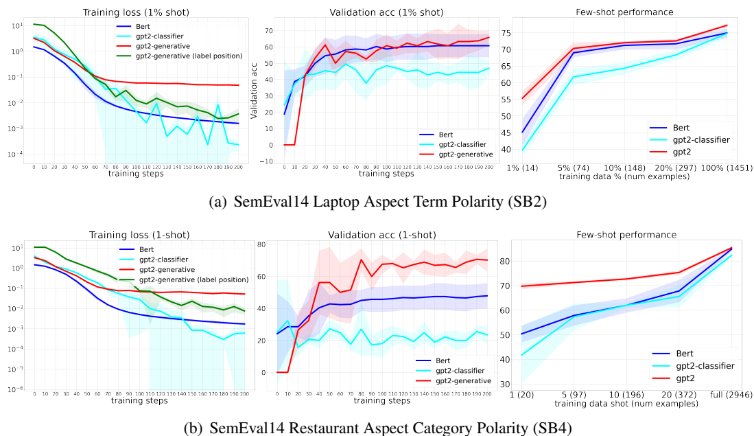
Figure 5: Analysis of few-shot training convergence, evaluated on SemEval14 for 1% and 1-shot training data, and few-shot performance on all settings (right). GPT2-classifier model uses a classification layer on the output of last input token without using language modeling loss for training. (best viewed in color)
