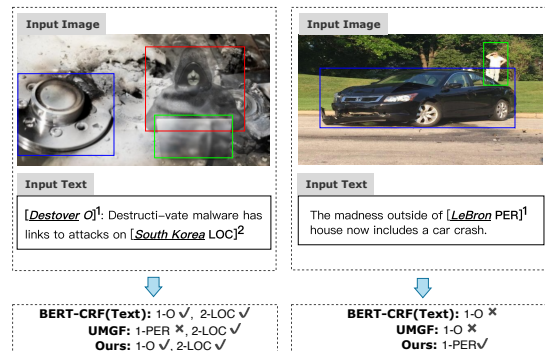
Figure 1: Motivation for robust and effective hierarchical modalities fusion.
