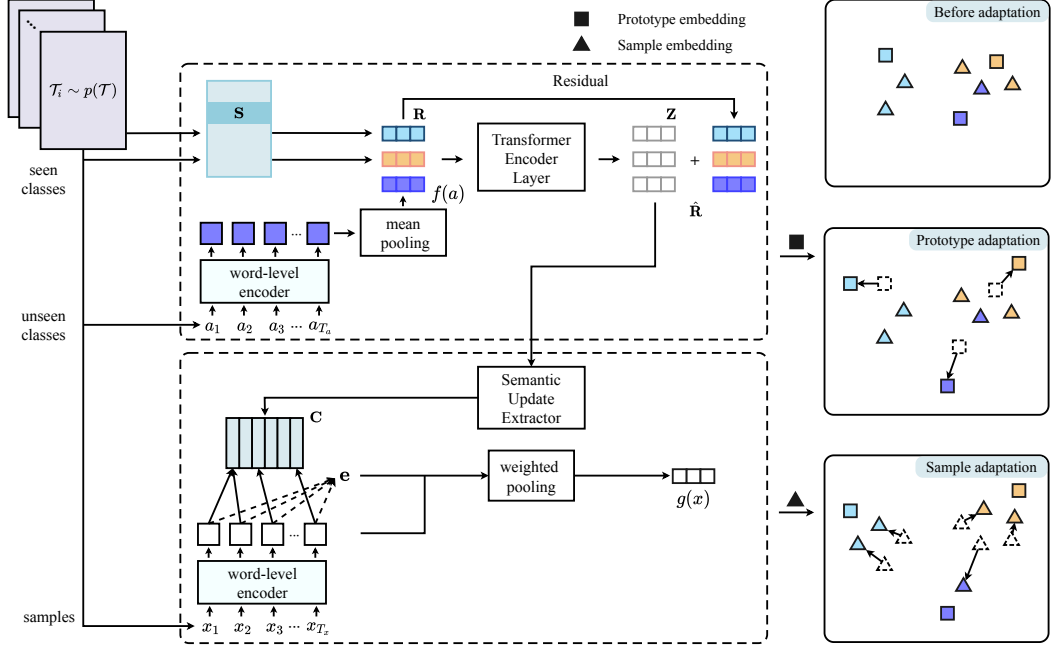
Figure 1: Illustration of the proposed LTA framework. The right part demonstrates the prototype adaptation and sample adaptation, in which \blacksquare and \blacktriangle respectively denote prototypes and samples, dotted border and solid border represent before and after adaptation, respectively.
