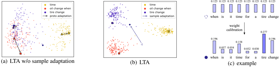
Figure 2: PCA plots of encoded unseen sample representations(·) and prototype representations(■) from (a) LTA w/o sample adaptation model and (b) full LTA model with sample adaptation (c) is an unseen example with sample-level raw attention and adapted attention. ▲ denotes the raw prototype before adaptation. ○ and ● respectively denote the example representations before and after sample adaptation.
