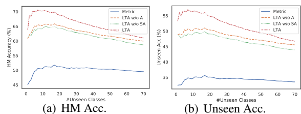
Figure 3: The performance with increasing numbers of test unseen classes on CLINC dataset.
