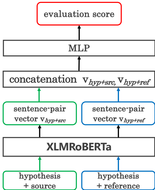
Figure 1: Architecture of C-SPEC
