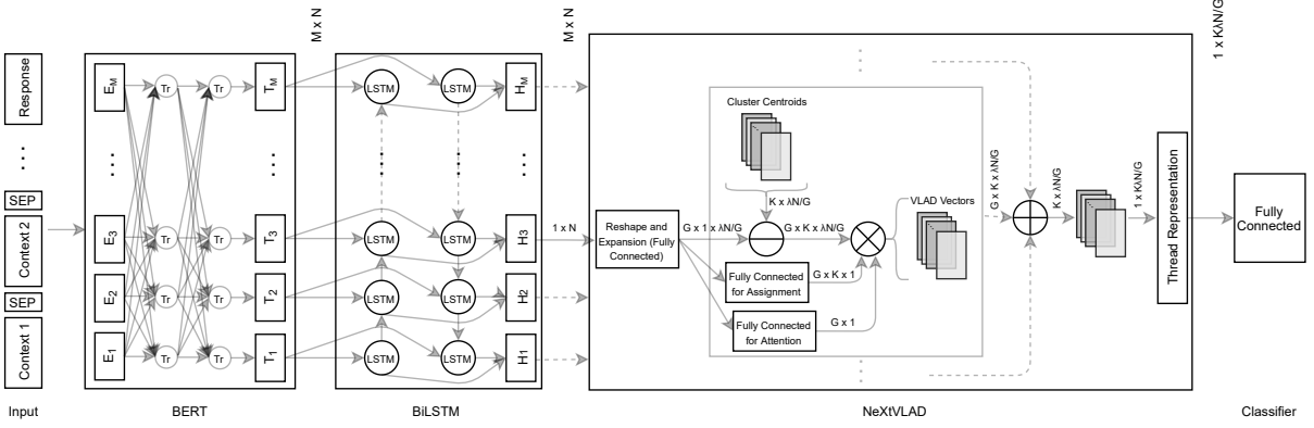
Figure 1: The architecture for sarcasm detection, where M is the number of tokens from the input text, N is the dimension of the BERT representation, and G is the number of groups into which the input is split after expansion.
